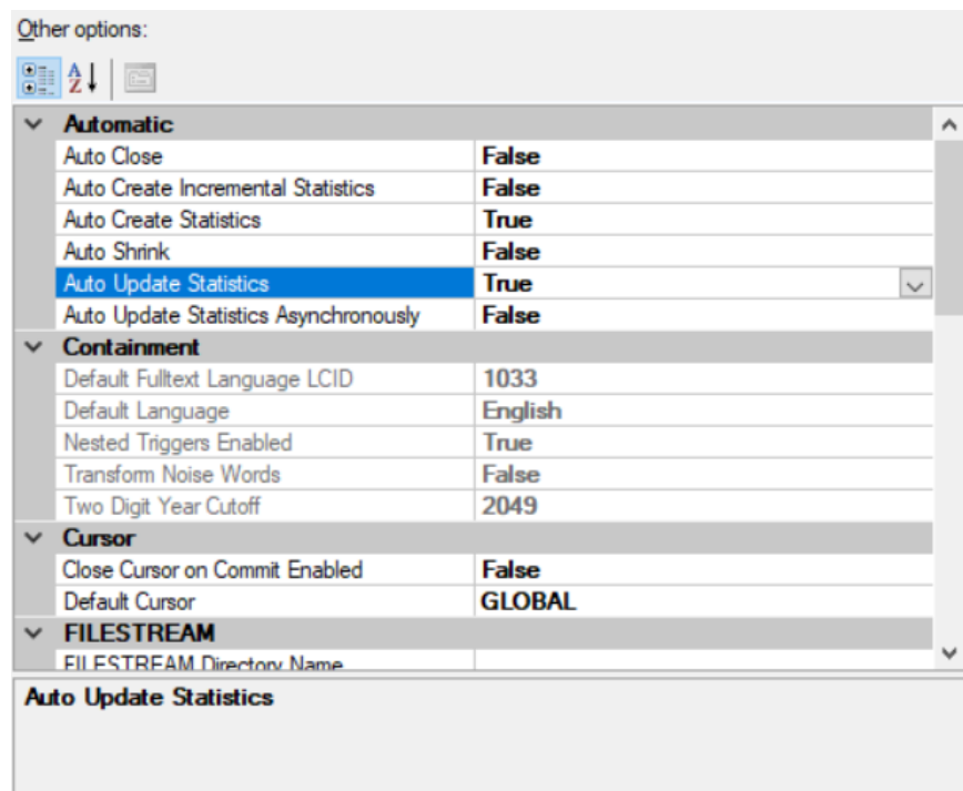
Figure 5: Database options
