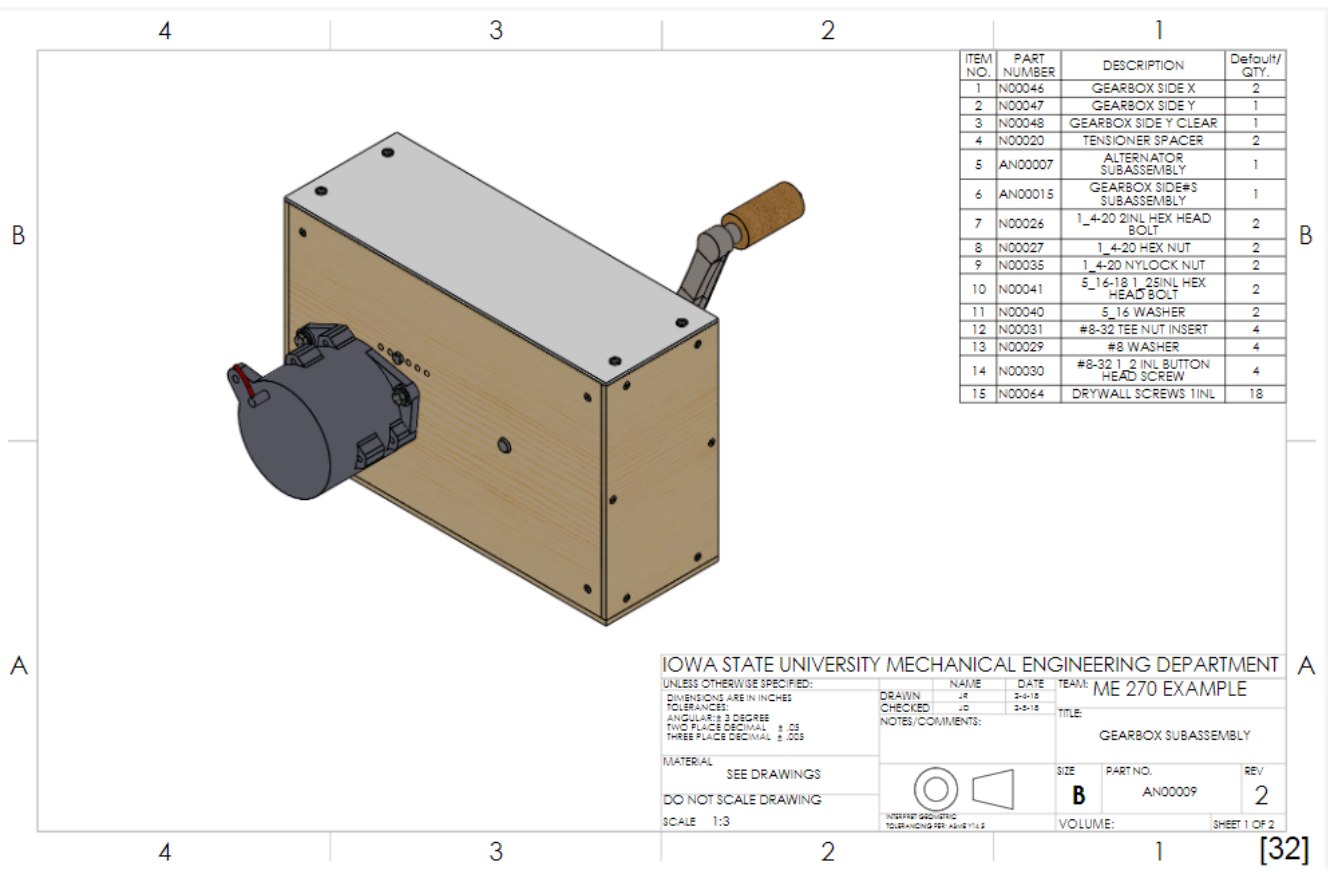
This picture/image shows a fully assembled gearbox engineering drawing example with bill of materials (BOM) in the upper right corner and title block in the lower right corner. Click on picture/image to review and/or download. Click on picture/image to review and/or download. I
